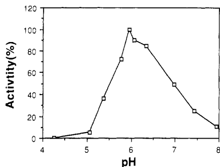
FIGURE 3: pH versus activity profile for RBG200 DHFR. The percentage of RBG200 DHFR activity is shown at different pH values. Potassium phosphate buffer, 50 mM, containing 1 mM EDTA and 1 mM DTT was used for the pH range 4.2–7.9. The pH was measured prior to, and immediately after, monitoring of the absorbance change of reaction with a microelectrode and found to vary less than \pm 0.05 unit. Each data point is the average of three separate assays.
